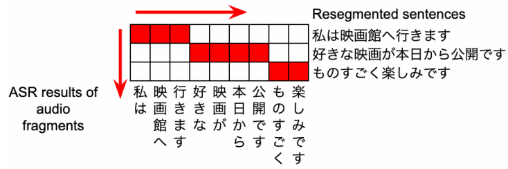
Figure 5 Example of Aligning using Dynamic Programming
