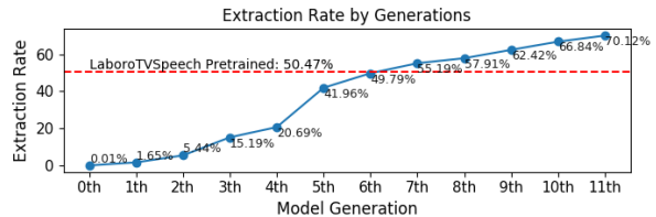
Figure 3 Extraction rate for every generation on one-day amount of unseen recordings
